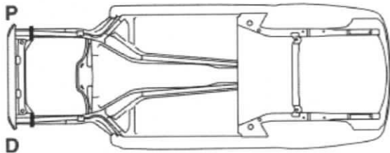
UNDERBODY VIEW
