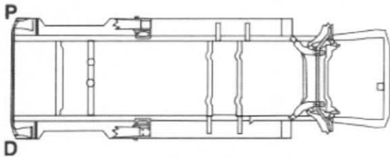
UNDERBODY VIEW
